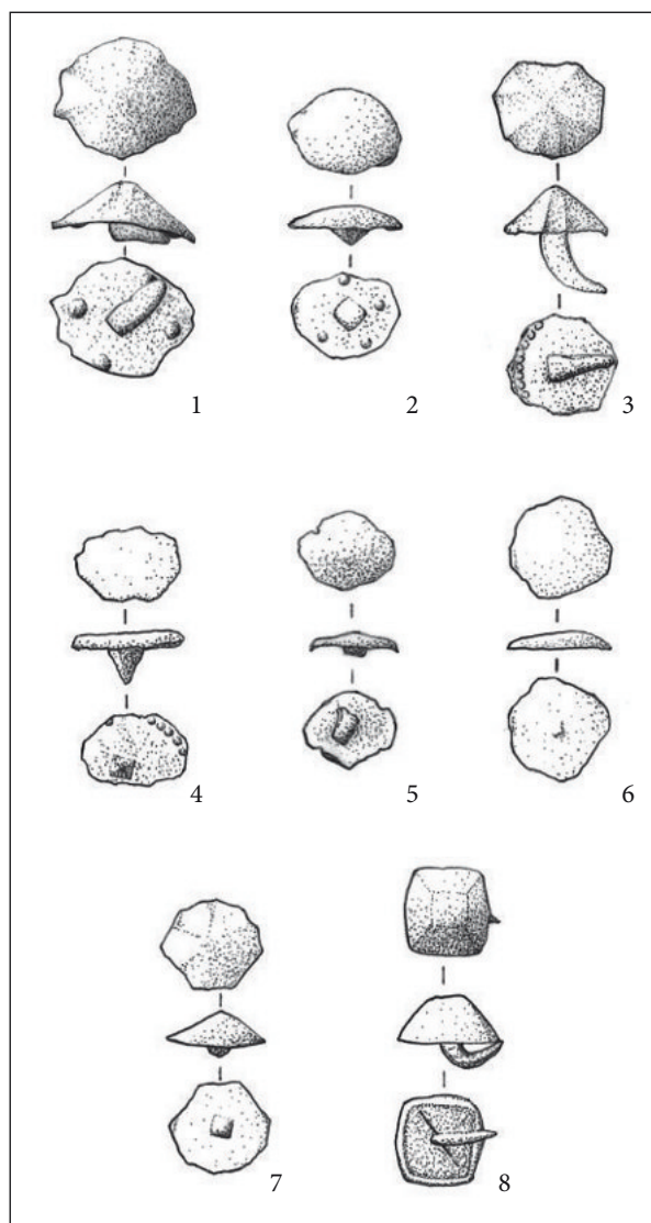
Fig. 4: Shoe hobnails from the site no. 3, above the Grozzana village. Scale = 1:1. Drawings by Andrea Fragiaco.
