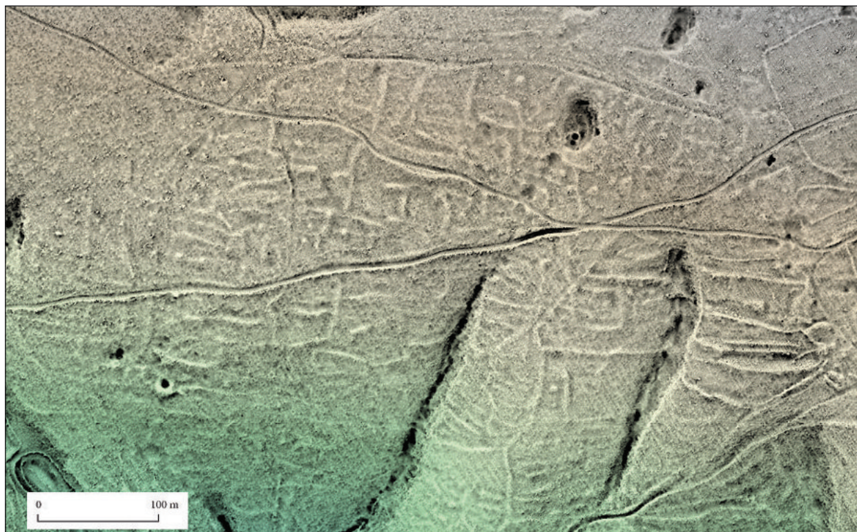
Fig. 3: Mandarje, 0.5 m LiDAR-derived digital elevation model revealing the remains of probable agricultural structures, which are not mapped in the examined historical and modern maps. Data processing and visualization by Edisa Lozić.
