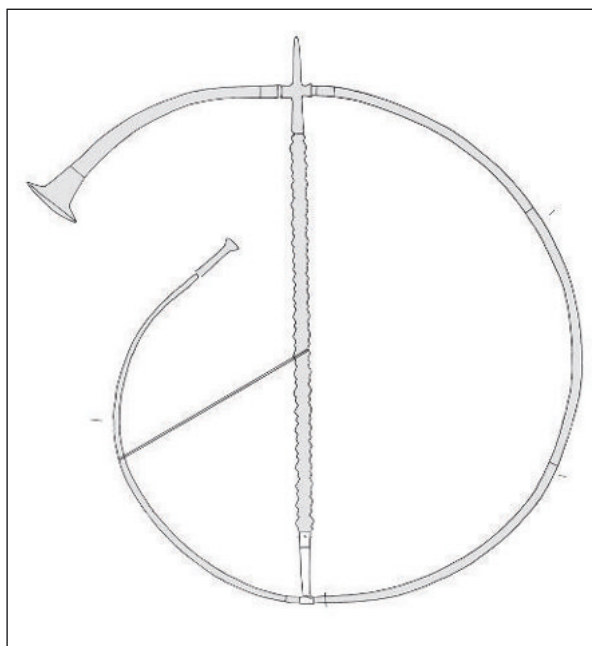
Fig. 9: Reconstruction of the cornu from Nadleški hrib. Not to scale. Drawing Ida Murgelj.
